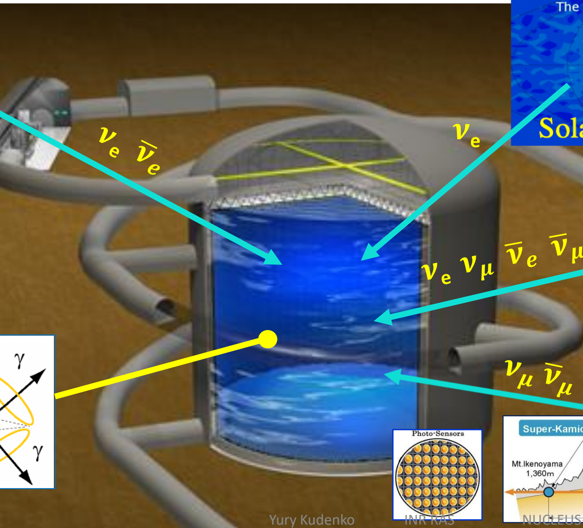
Atmospheric neutrinos
